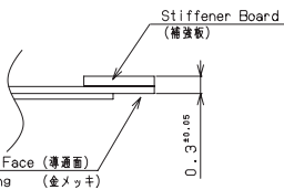
Contact Sectioning View (コネクタ断面図)
